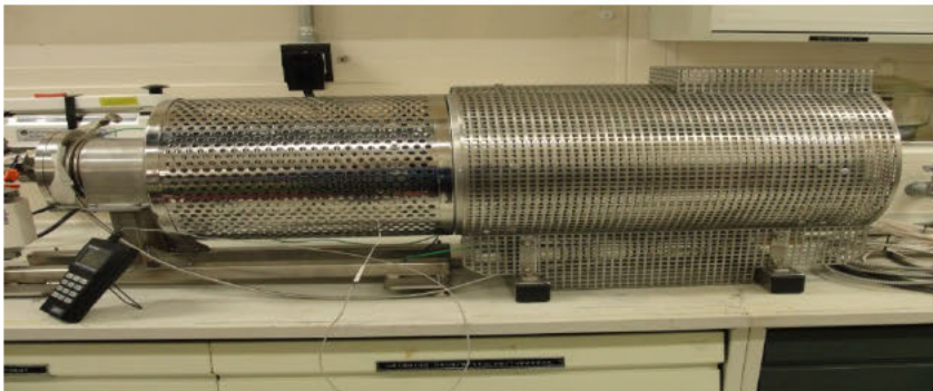
Vacuum Salt Distillation Equipment for HBL
