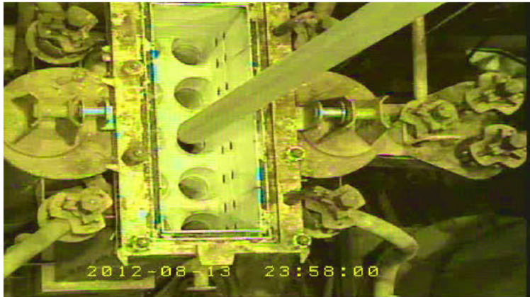
Spent Fuel Charging to Dissolver
